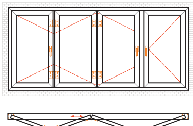
SLIDE & FOLD DOOR-431 INWARD OPENING
