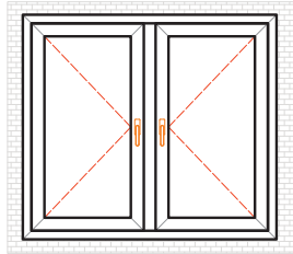
CASEMENT DOOR-DOUBLE OPEN OUTWARD OPENING
