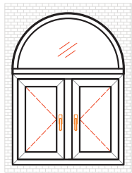
CASEMENT WINDOW-DOUBLE OPEN WITH TOP FIX-ARCH (OUTWARD OPENING)
