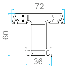
AP 206 T MULLION
