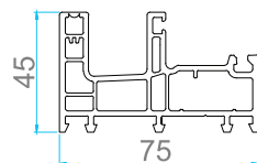
AP 212 UP-STAND BEAD
