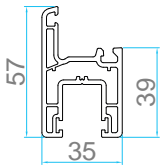
AP 604 SLIDING WINDOW SASH
