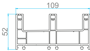
AP 103 SLIDING FRAME 3-TRACK
