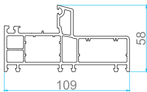
AP 401 VILLA WINDOW OUTER FRAME
