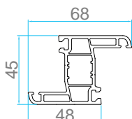
AP 707 CASEMENT Z-MULLION
