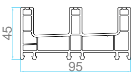
AP 603 SLIDING FRAME 3 - TRACK
