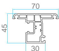
AP 704 CASEMENT WINDOW SASH
