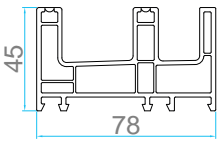
AP 602 SLIDING FRAME WITH MESH TRACK
