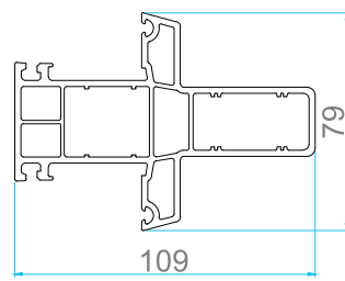
AP 406 TRANSOM / MULLION
