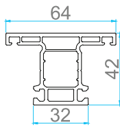
AP 107 T MULLION FOR SLIDING
