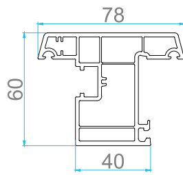
AP 204 CASEMENT WINDOW SASH
