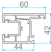
AP 104 SLIDING WINDOW SASH
