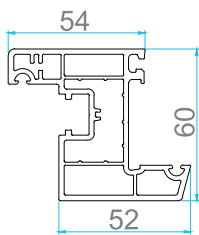
AP 214 INWARD WINDOW SASH
