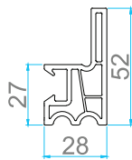
AP 115 ADD. TRACK FOR MESH
