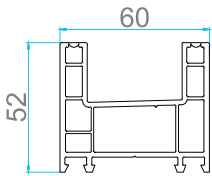
AP 101 SLIDING FRAME 2-TRACK
