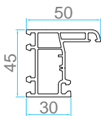
AP 701 CASEMENT OUTER FRAME
