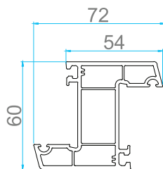
AP 207 Z MULLION
