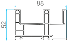
AP 102 SLIDING FRAME WITH MESH TRACK
