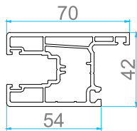
AP 114 SLIDING INTERMEDIATE SASH
