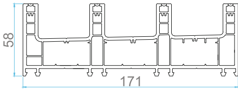
AP 303 SLIDING FRAME 4-TRACK
