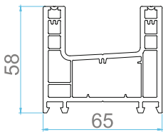
AP 301 SLIDING FRAME 2-TRACK
