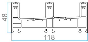
AP302 A SLIDING INTERMEDIATE FRAME 3 -TRACK
