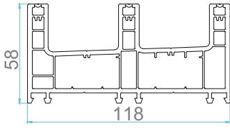
AP 302 SLIDING FRAME 3-TRACK
